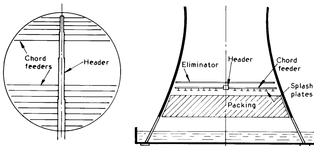
(b) Diametric header, chord feed
