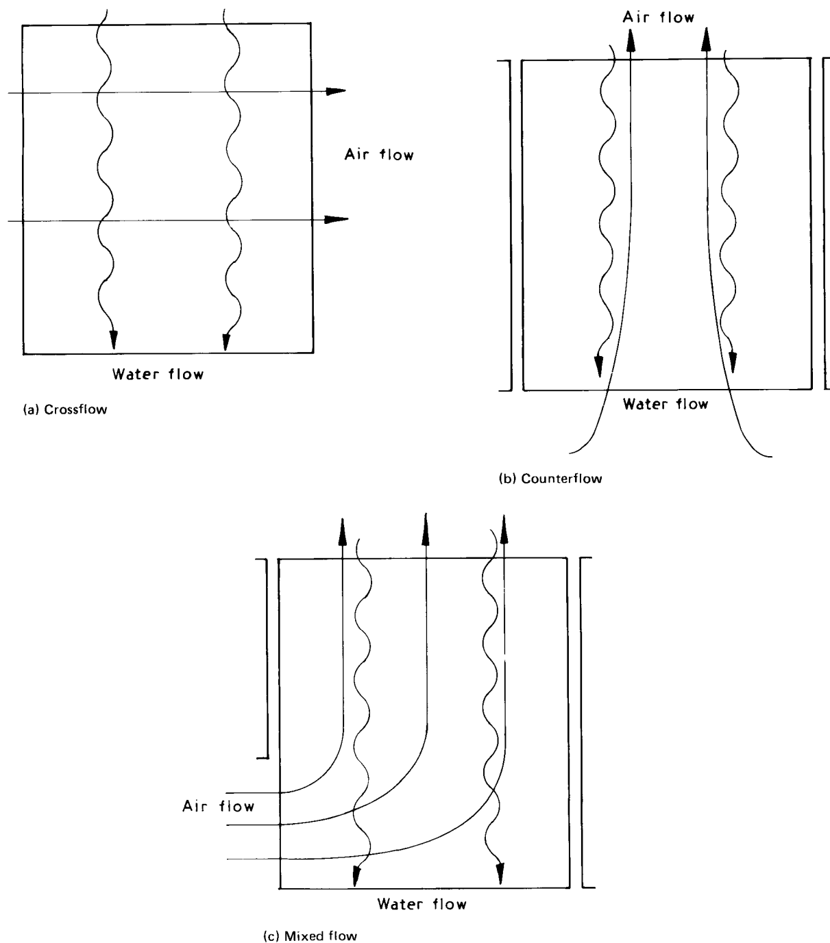
Figure 1 — Air-water flow paths in crossflow, counterflow and mixed flow towers
