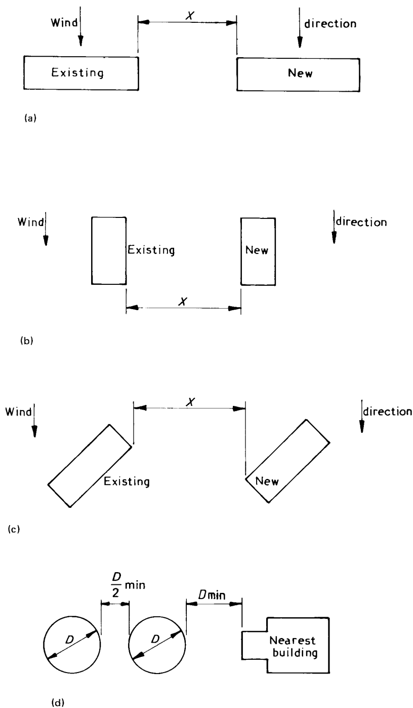
Figure 8 — Spacing
