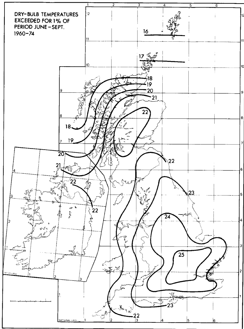
(a) Dry bulb temperatures exceeded for 1 % of hours.
