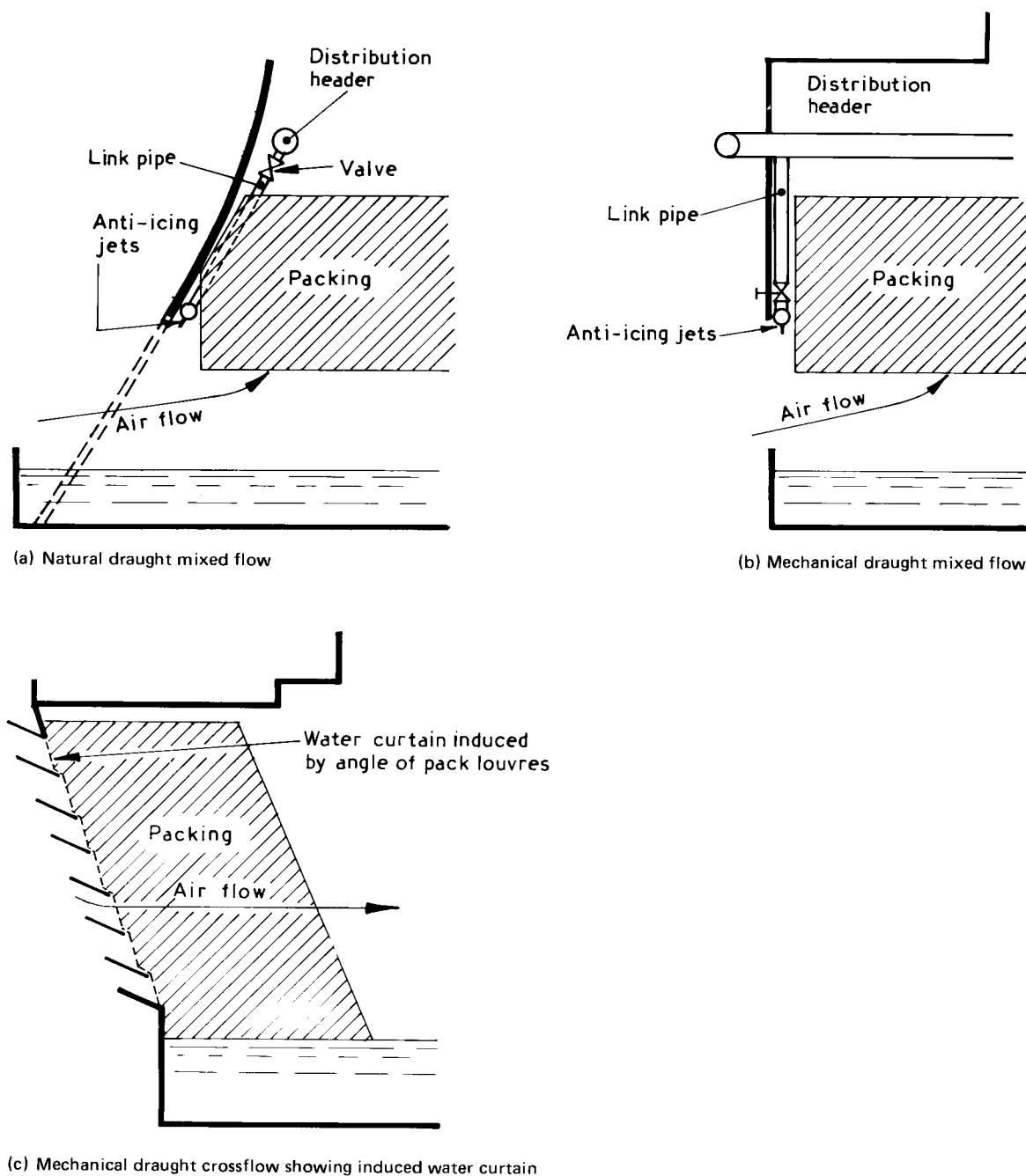
Figure 23 — Anti-icing arrangements
