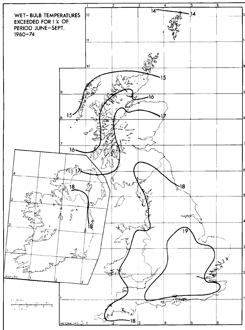
(c) Wet bulb temperatures exceeded for 1 % of hours.
