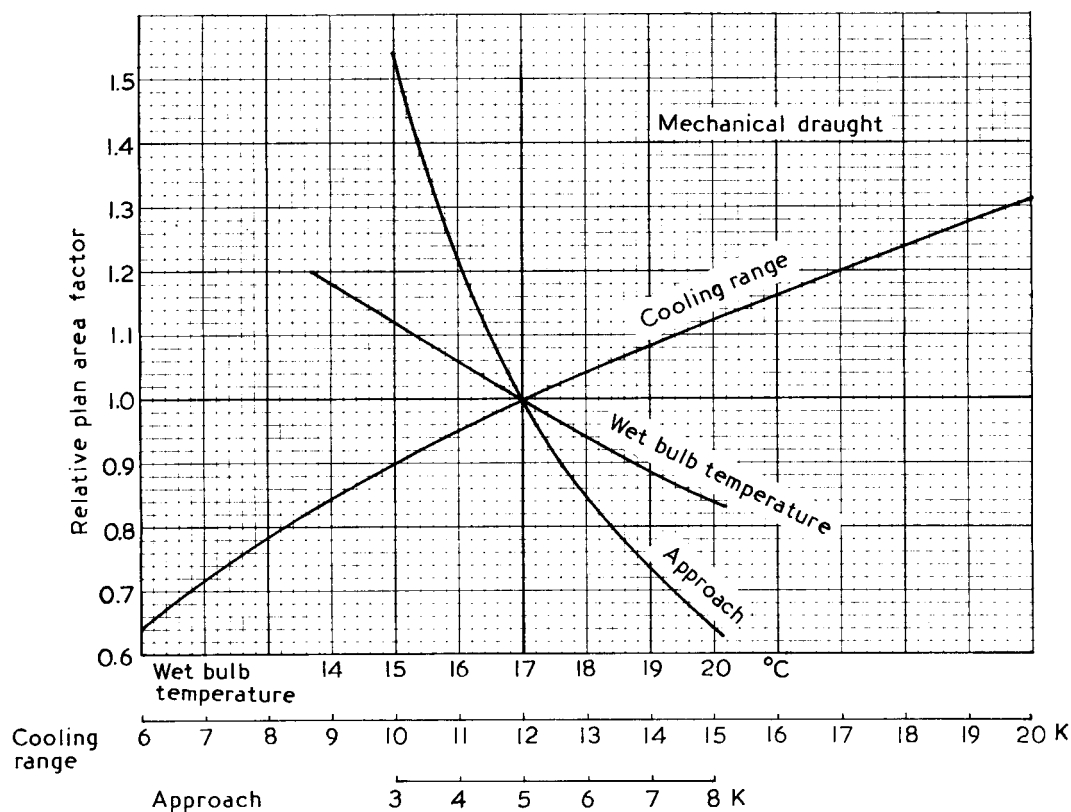
Figure 10 — Mechanical draught counterflow tower: variation of tower size with cooling range, approach and wet bulb temperature
