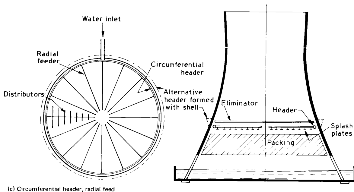
Figure 17 — Natural draught tower: water distribution
