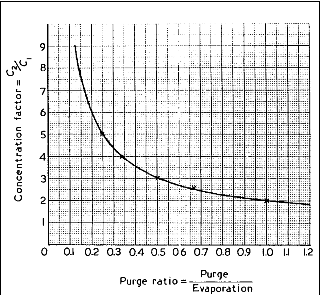
Figure 21 — Relation between purge ratio and concentration factor
