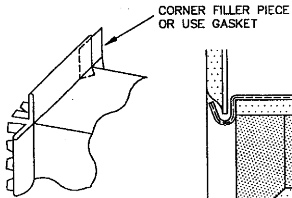
CLINCH LOCK
