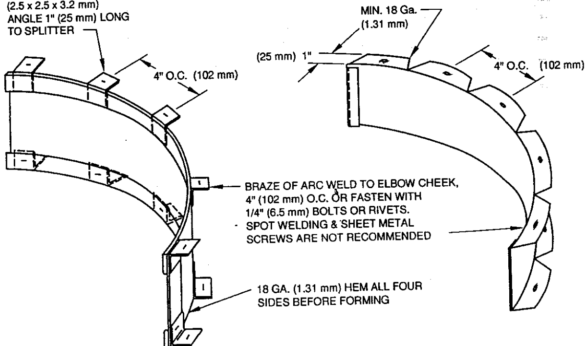
SPLITTER DETAIL
