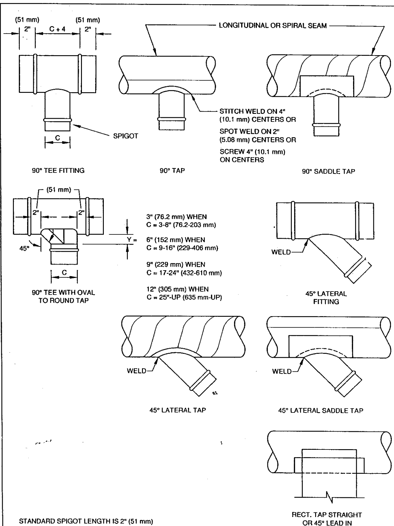
90° TEES AND LATERALS
