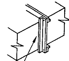
ANGLE TIE 1"x1"x12 GA. (2.5 X 2.5 X 2.75 mm) MINIMUM
