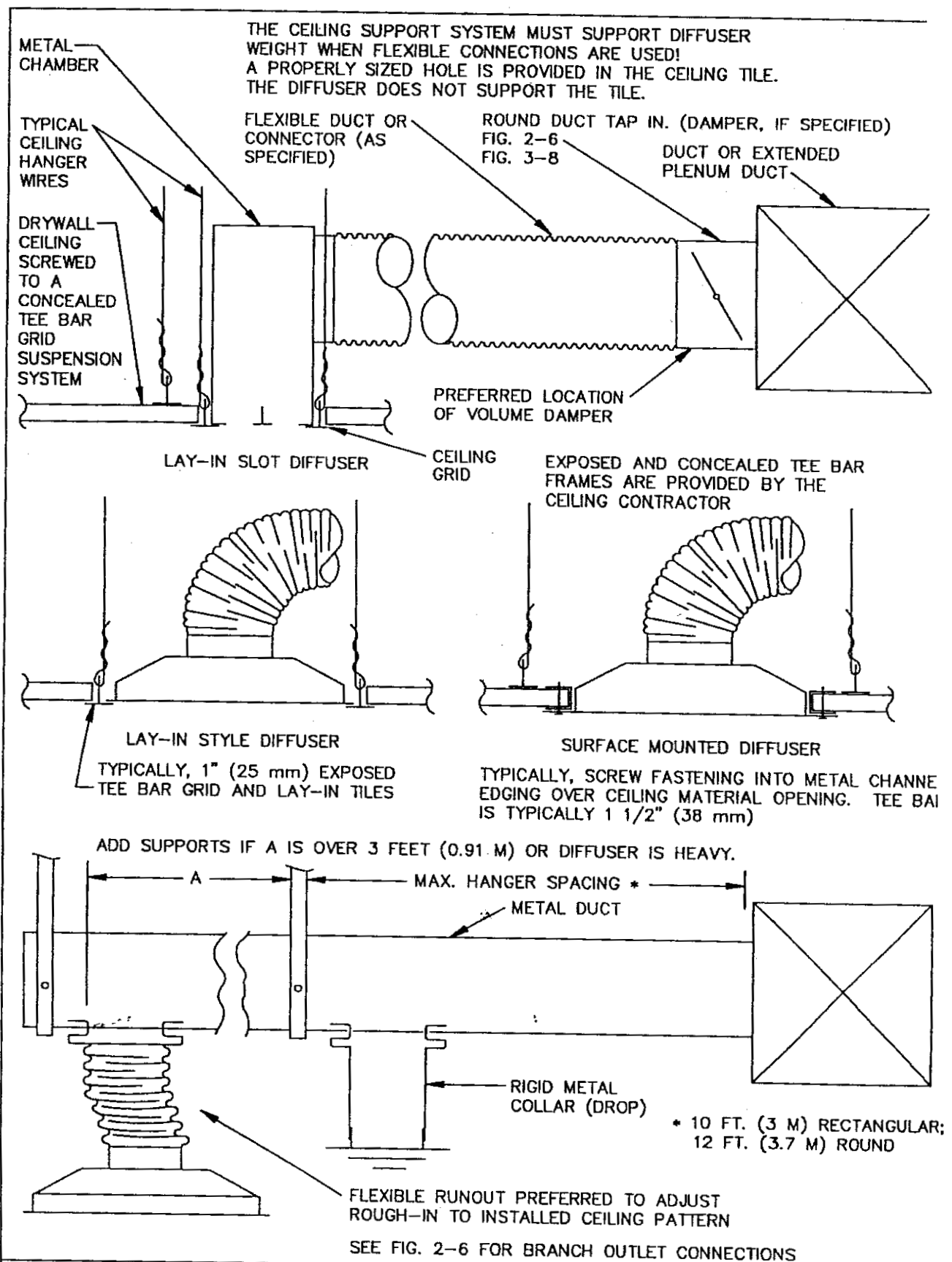
CEILING DIFFUSER BRANCH DUCTS
