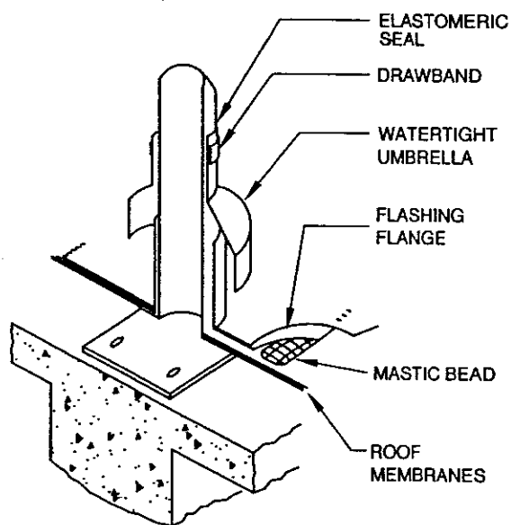
CONCRETE DECK
