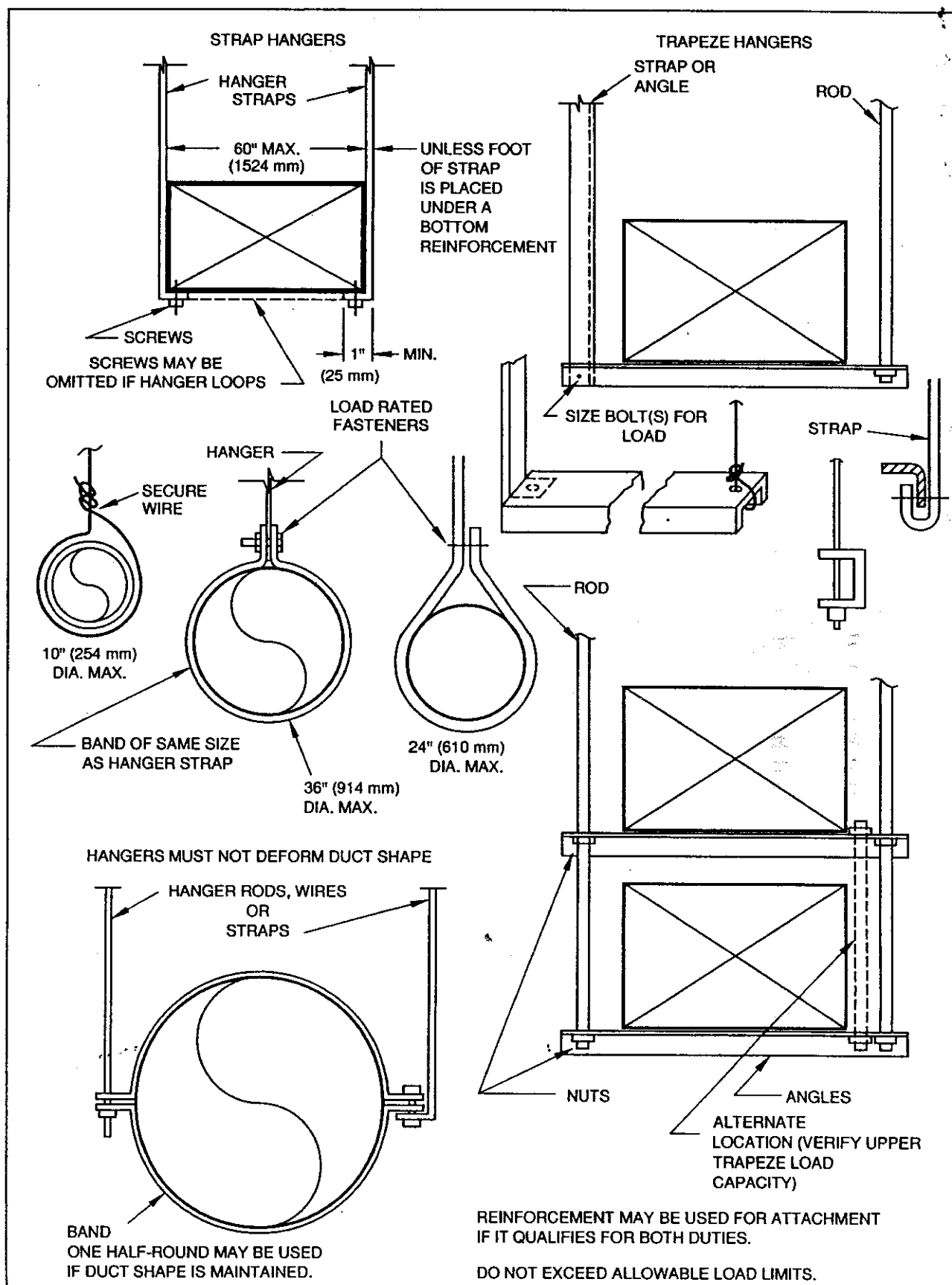
LOWER HANGER ATTACHMENTS
