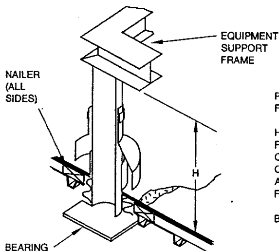
INSULATED STEEL DECK
