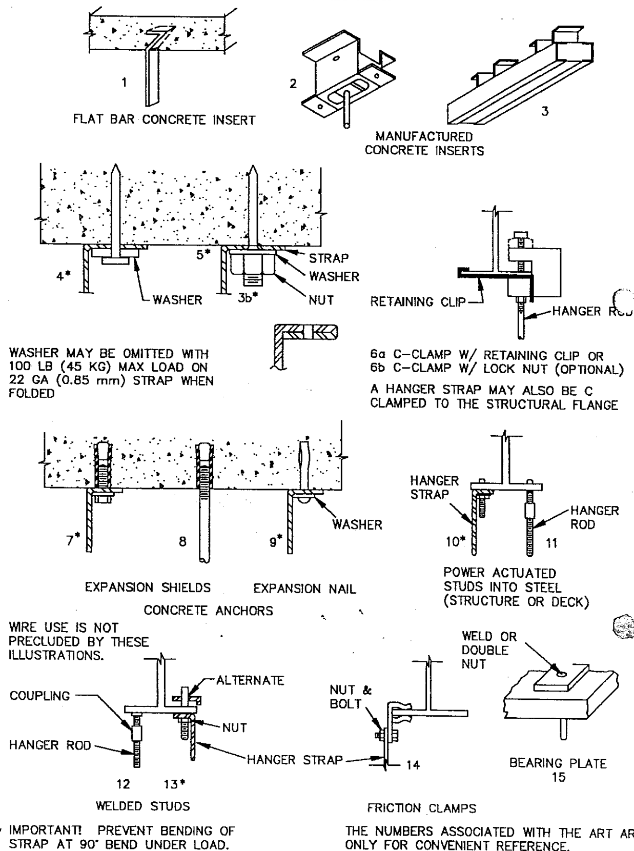
UPPER ATTACHMENT DEVICES - TYPICAL
