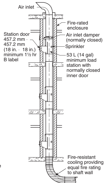
FIGURE A.21.15.2.2(d) Fire Damper Engineering Alternative for Penetration of Floor at Base of Shaft. [82:Figure A.5.3(b)]
