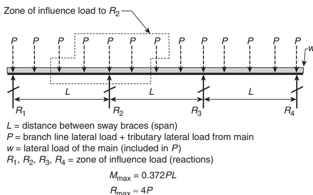
FIGURE E.2.2(c) Maximum Demands for Spans of 40 ft.
