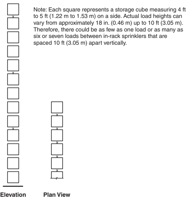
FIGURE 16.3.4.1.2.1(b) Class I, Class II, or Class III Commodities, In-Rack Sprinkler Arrangement, Single-Row Racks, Storage Height Over 25 ft (7.6 m) — Option 1.
