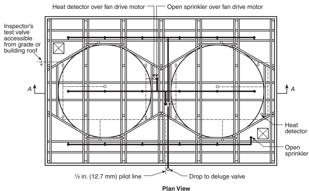
FIGURE A.21.21.2.1(a) Plan View, Typical Deluge Fire Protection Arrangement for Counter-flow Towers. [214:Figure A.5.2.4.1(a)]
