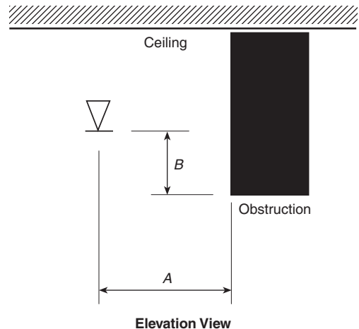
FIGURE 8.8.5.1.2(a) Position of Sprinklers to Avoid Obstructions to Discharge (Extended Coverage Upright and Pendent Spray Sprinklers).
