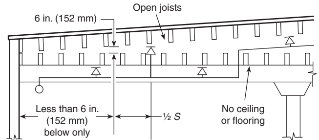
FIGURE 8.6.4.1.5.1 Arrangement of Sprinklers Under Two Sets of Open Joists — No Sheathing on Lower Joists.
