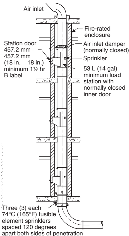
FIGURE A.21.15.2.2(d) Fire Damper Engineering Alternative for Penetration of Floor at Base of Shaft. [82:Figure A.5.3(b)]
