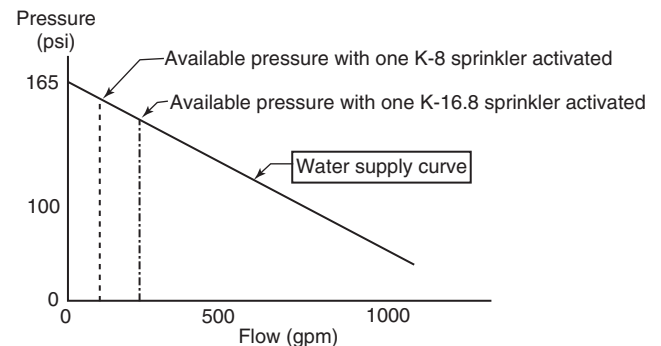
FIGURE A.12.6 Available Pressure Comparison.
