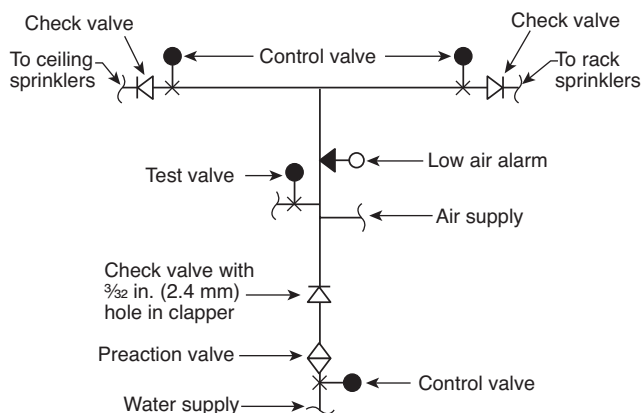
FIGURE 7.9.2.8.4 Valve Arrangement.
