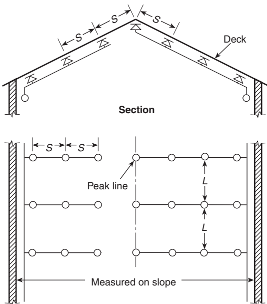
FIGURE 8.10.3.5(a) Maximum Distance Between Sprinklers with Sloped Ceilings — Arrangement A.
