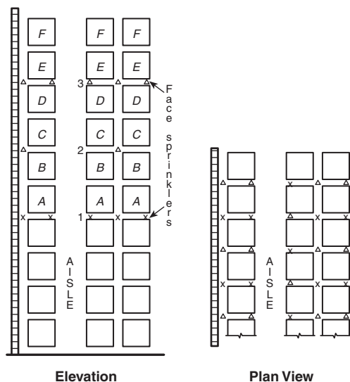
FIGURE 16.3.4.1.1.1(b) In-Rack Sprinkler Arrangement, Class I Commodities, Storage Height Over 25 ft (7.6 m).
