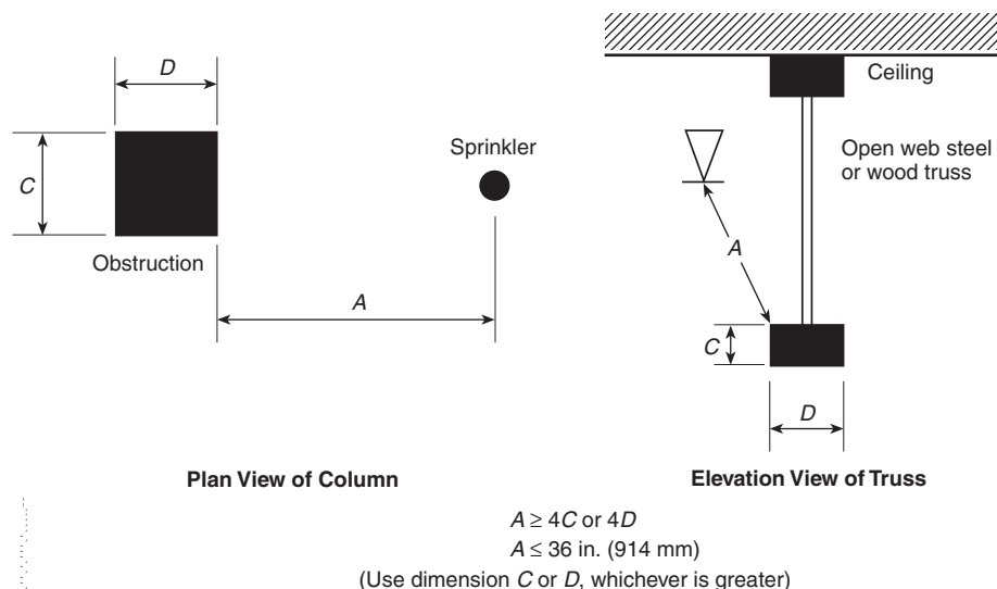
FIGURE 8.10.6.2.1.3 Minimum Distance from Obstruction (Residential Upright and Pendent Spray Sprinklers).
