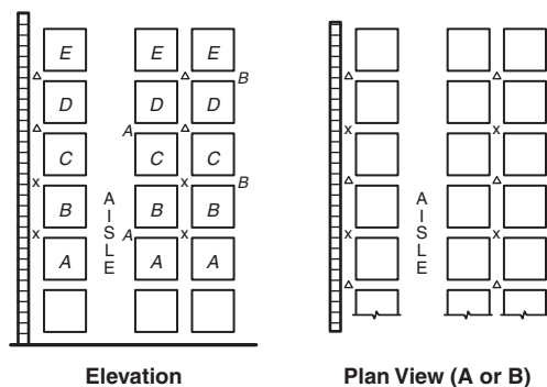
FIGURE 16.3.4.1.1.1(c) In-Rack Sprinkler Arrangement, Class I, Class II, or Class III Commodities, Storage Height 25 ft to Maximum 30 ft (7.6 m to Maximum 9.1 m).
