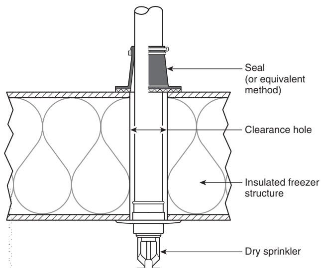
FIGURE A.8.4.9.2(a) Dry Sprinkler Seal Arrangement — Seal on Exterior of Freezer Structure.
