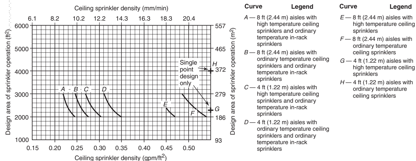
FIGURE 16.2.1.3.2(e) Single- or Double-Row Racks — 20 ft (6.1 m) High Rack Storage — Class I and Class II Encapsulated Commodities — Conventional Pallets.
