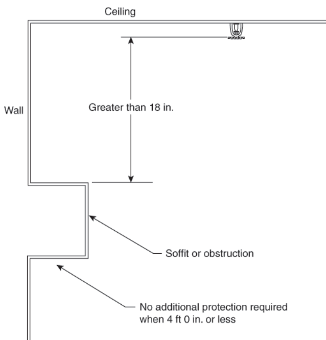
FIGURE A.8.6.5.1.2 Soffit/Obstruction Against Wall Greater Than 18 in. Below Deflector.
