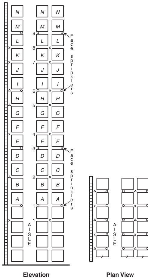
FIGURE 16.3.4.1.1(h) In-Rack Sprinkler Arrangement, Class I, Class II, Class III, or Class IV Commodities, Storage Height Over 25 ft (7.6 m) — Option 1.
