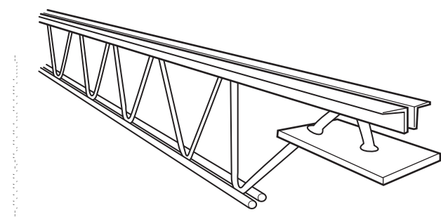
FIGURE A.3.7.2(b) Open-Web Bar Joist Construction.
