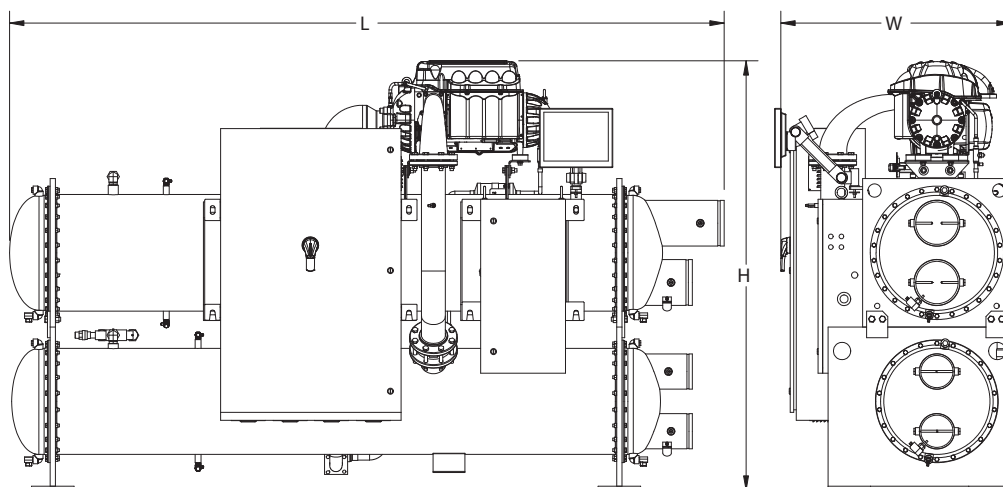
Figure 5: WMC145-400D (2-pass, right-hand configuration, with grooved connections)
