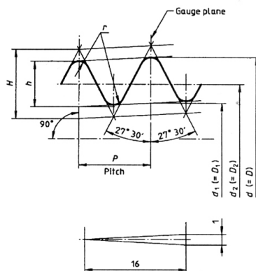
Taper thread
