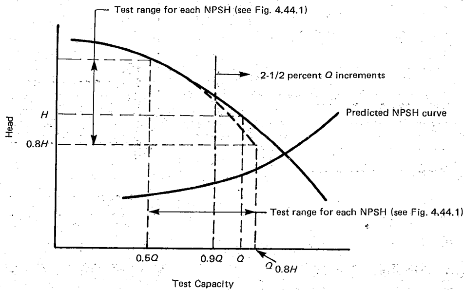
FIG. 4.44.2 CONSTANT NPSH
