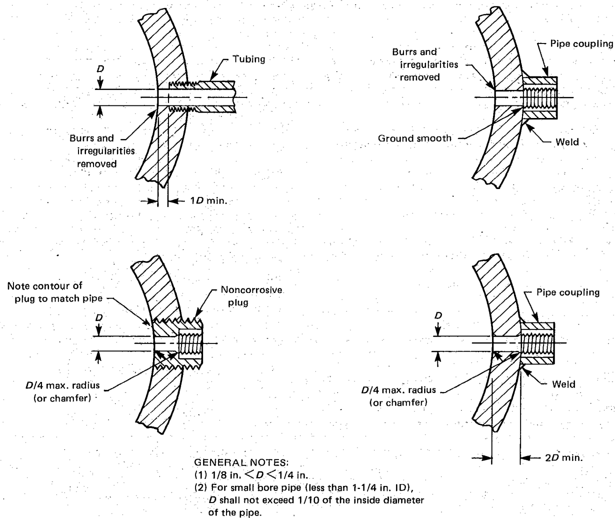
FIG. 4.7.1 TYPICAL PRESSURE TAP CONNECTIONS
