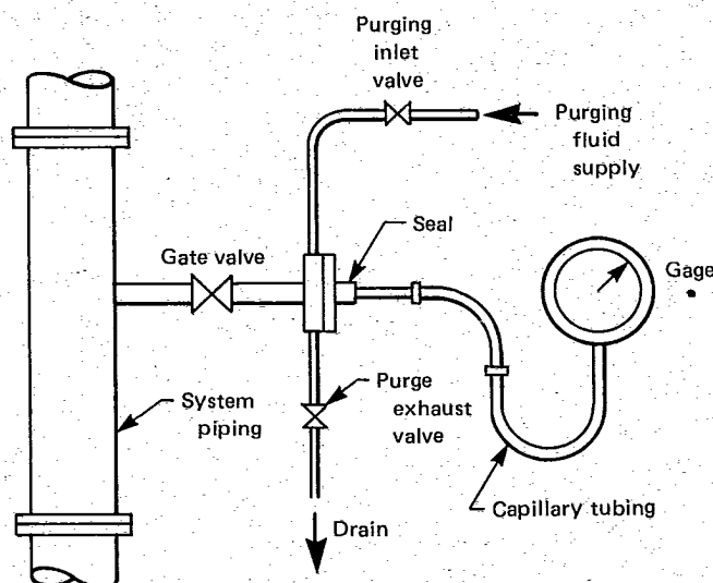
FIG. 4.12.2 A TYPICAL SEAL WITH INTERMITTENT PURGE
