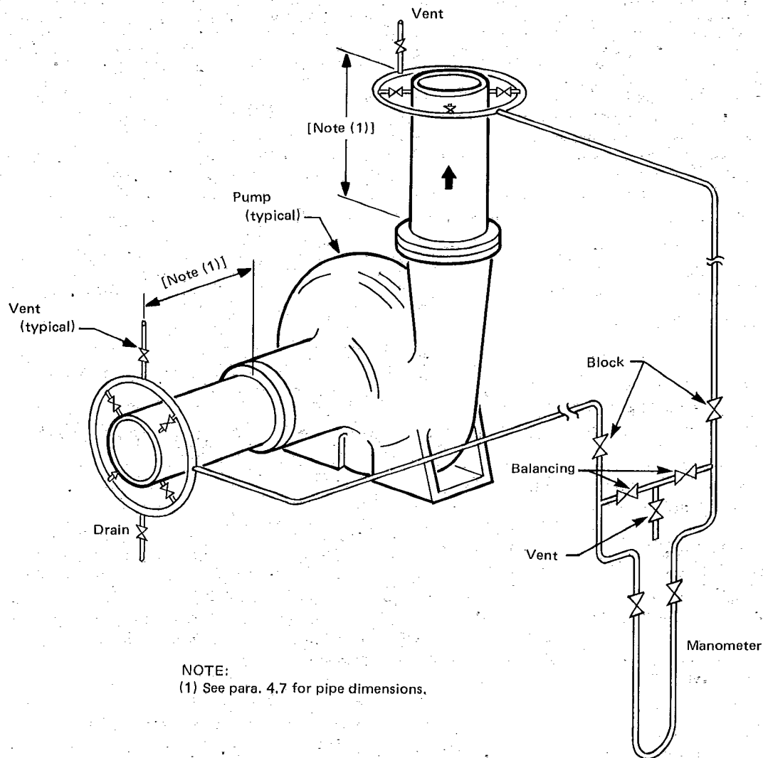
FIG. 4.7.7 TYPICAL PIEZOMETER RING MANIFOLD ARRANGEMENT FOR MEASUREMENT OF HEAD USING A DIFFERENTIAL MANOMETER
