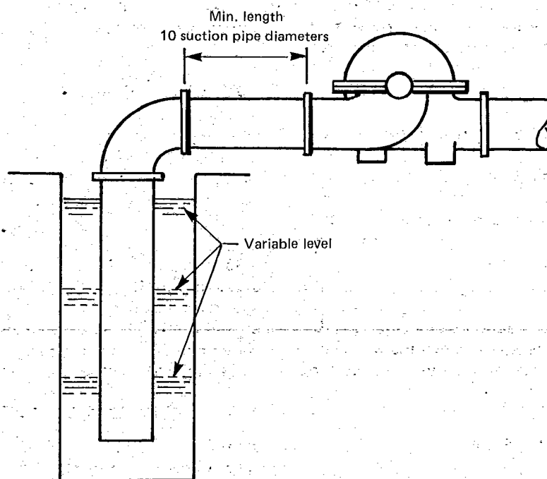
FIG. 4.40.1 NPSH TEST ARRANGEMENT
