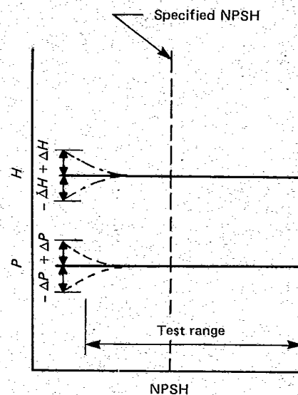
FIG. 4.43.3 CONSTANT CAPACITY
