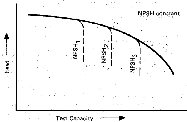
FIG. 4.44.1 CONSTANT NPSH
