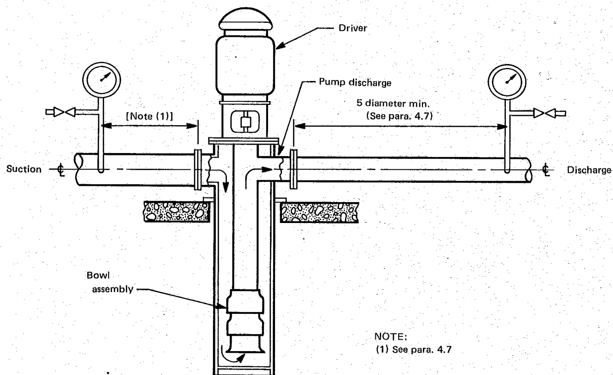
FIG. 4.7.3 TYPICAL PRESSURE TAP ARRANGEMENT FOR A VERTICAL CANNED SUCTION PUMP
