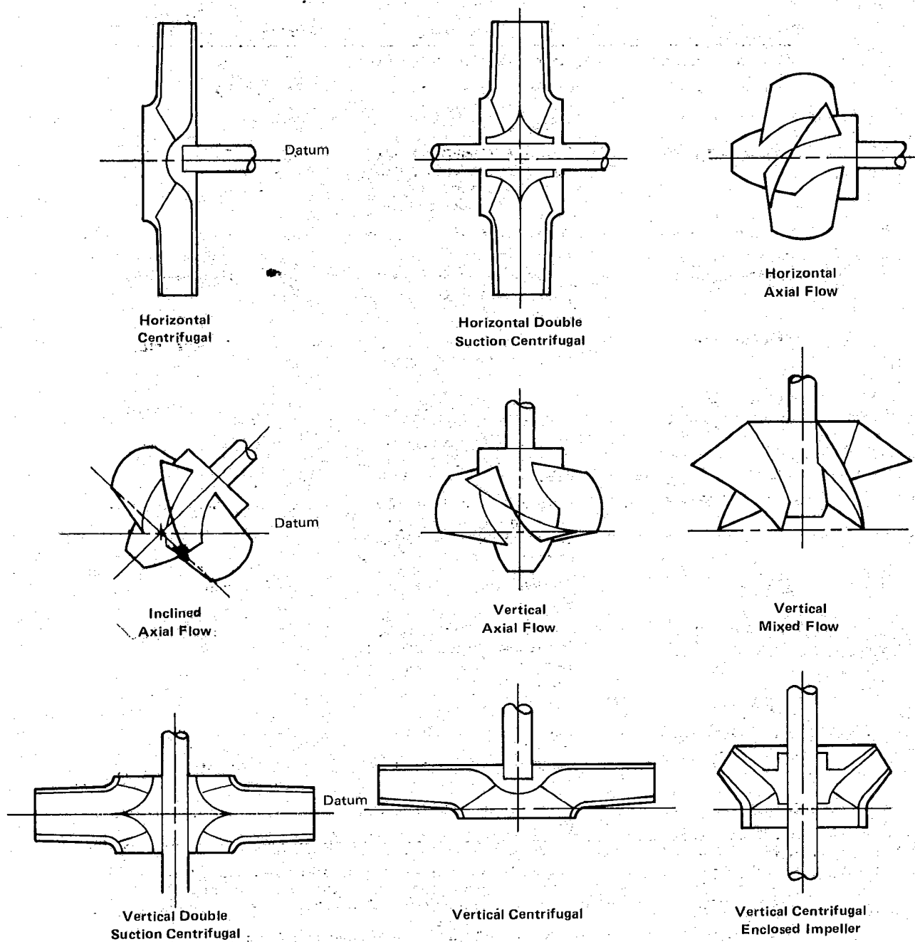
FIG. 2.2 DATUM LOCATION FOR TYPICAL PUMP TYPES
