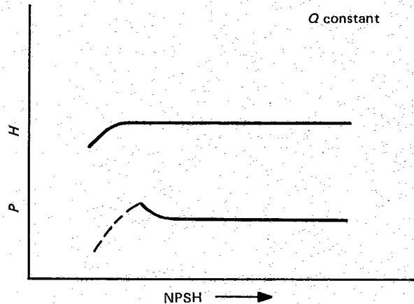
FIG. 4.43.2 CONSTANT CAPACITY
