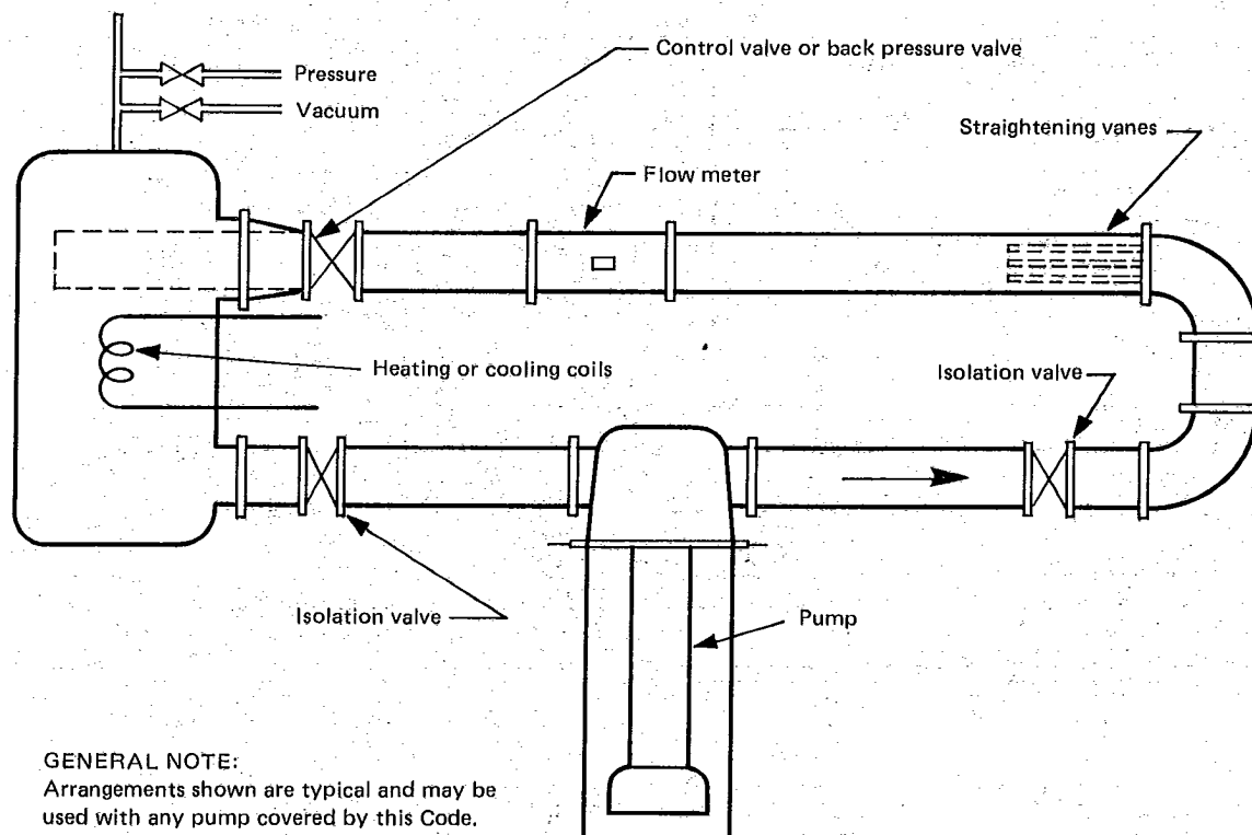
FIG. 4.40.4 NPSH TEST ARRANGEMENT
