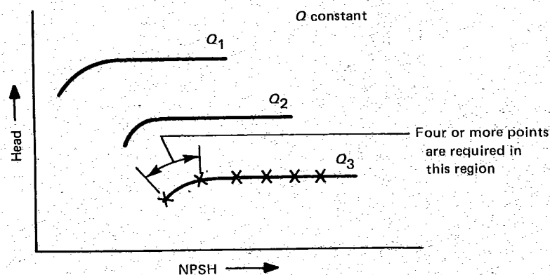
FIG. 4.43.1 CONSTANT CAPACITY
