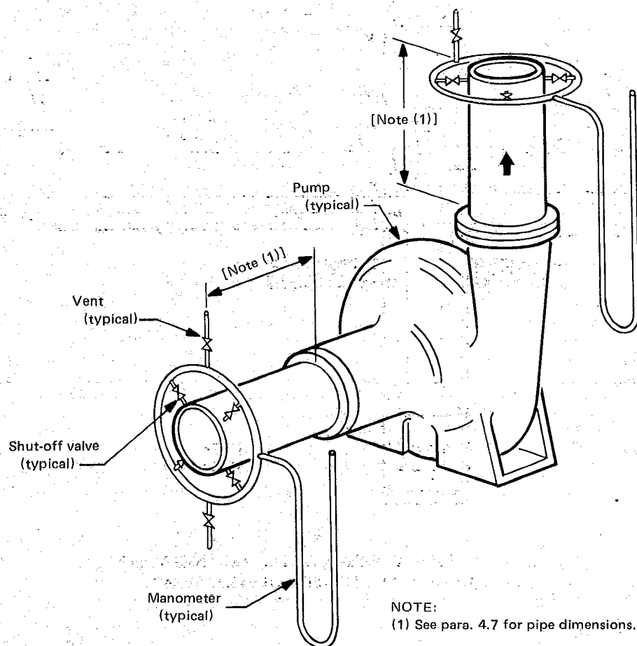
FIG. 4.7.4 TYPICAL PIEZOMETER RING MANIFOLD ARRANGEMENTS FOR MEASUREMENTS OF HEAD USING GAGES OR MANOMETERS
