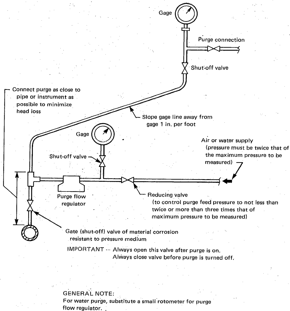
FIG. 4.12.1 A TYPICAL AIR OR WATER PURGE SYSTEM
