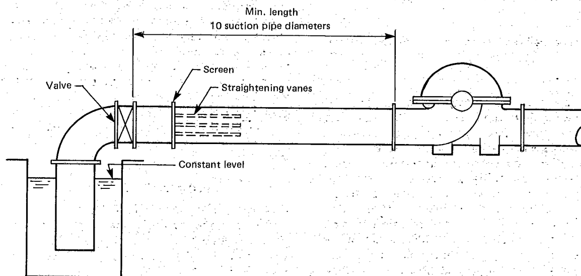
FIG. 4.40.2 NPSH TEST ARRANGEMENT
