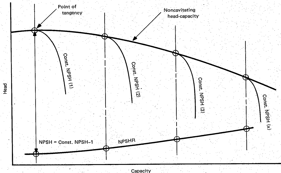
FIG. H3 NPSH TEST RESULTS FOR CONSTANT NPSH VALUES
