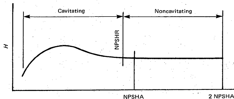
FIG. H2.1 GENERAL NPSH VS. HEAD PERFORMANCE (CONSTANT CAPACITY)
