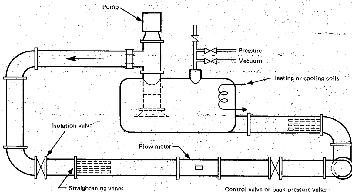
FIG. 4.40.3 NPSH TEST ARRANGEMENT
