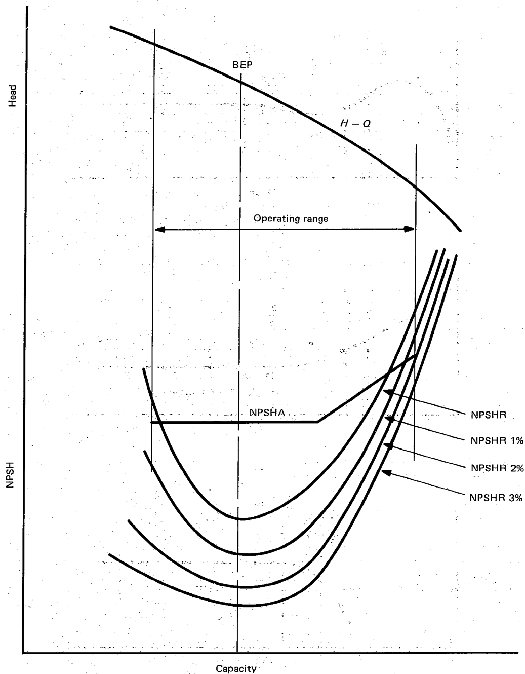
FIG. H2.3 NPSHR AT BREAK-OFF AND ALTERNATE HEAD REDUCTIONS
