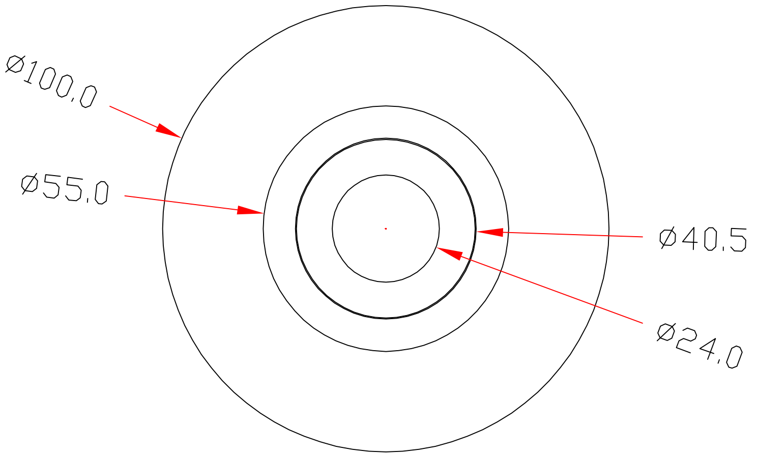
Inlet nozzle Aquamarine model WSP58
