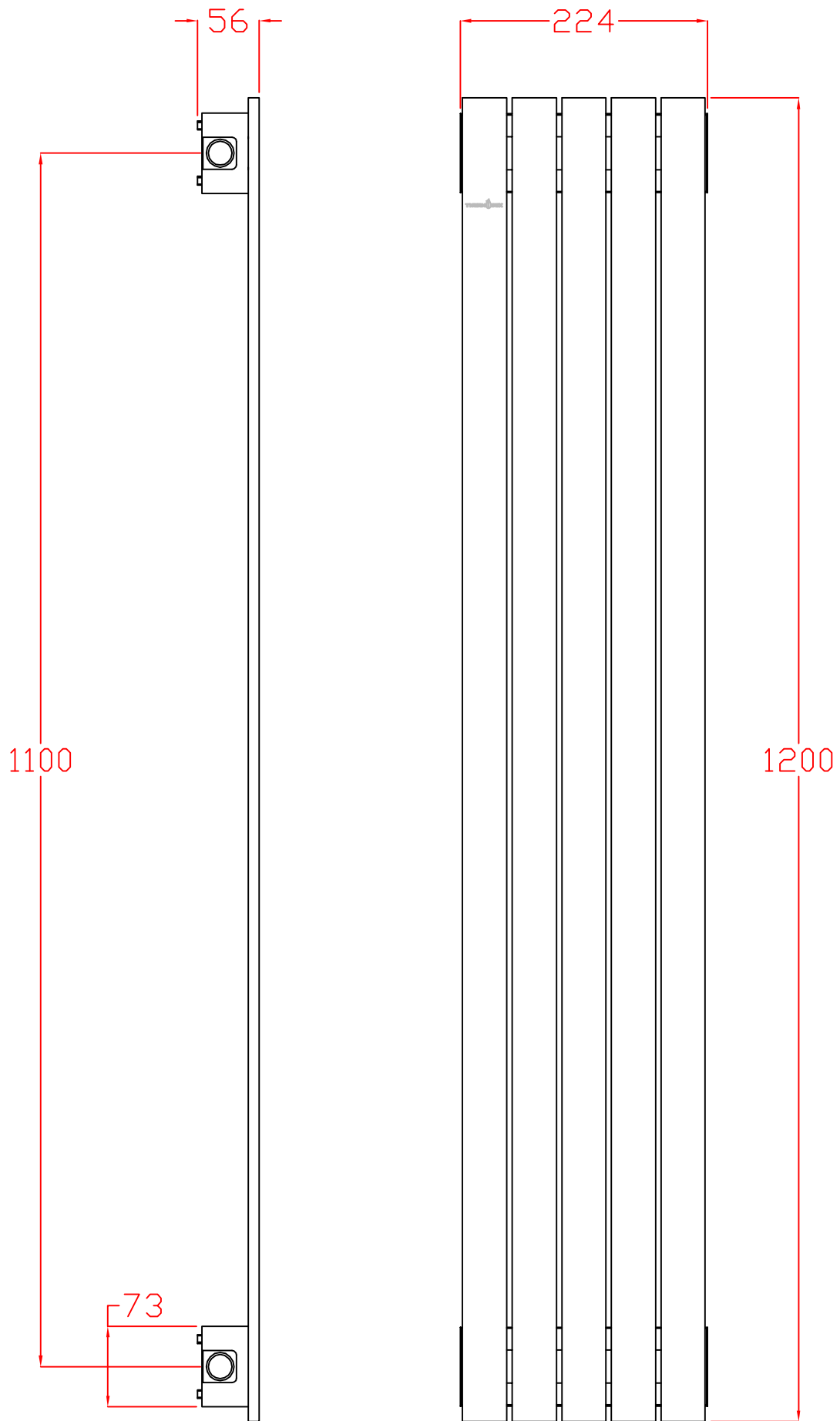
Thermobox ® TX5L dimensions
