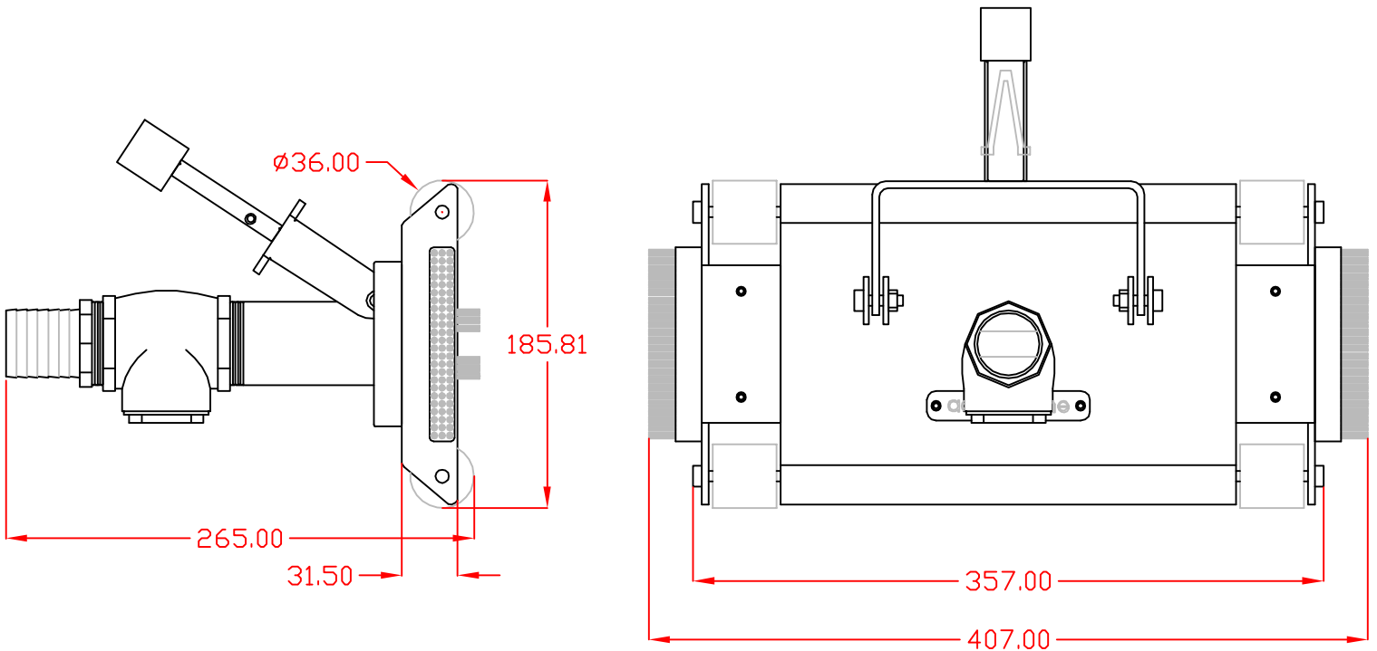
Aquamarine ® Air Vent sweeper head dimensions
